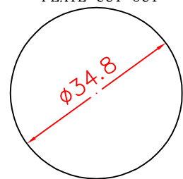
PB9按钮装配孔 PLATE CUT OUT
